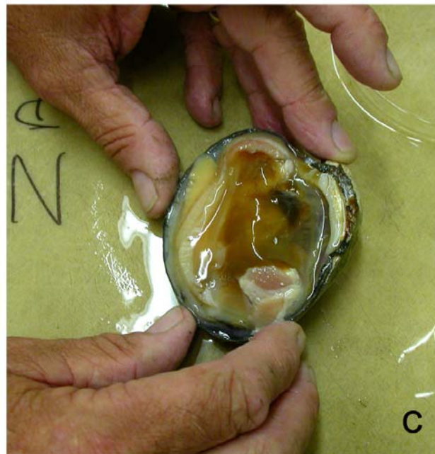
Text-figure 3. Collecting and extracting gut content samples for palynological processing. A. Collecting hard clams from the McQueen Locality. B. Opening an Atlantic ribbed mussel shell. C. Hard clam body before dissection of gut contents. D. Gut contents of hard clam placed in glass beaker, ready for chemical treatment.
