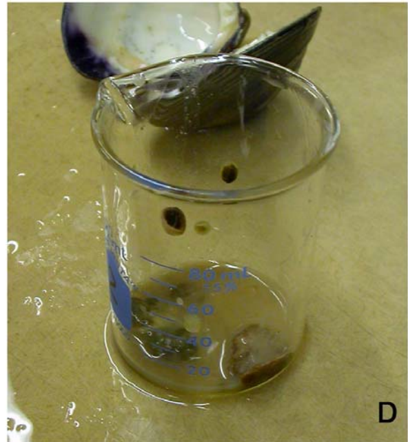
Text-figure 3. Collecting and extracting gut content samples for palynological processing. A. Collecting hard clams from the McQueen Locality. B. Opening an Atlantic ribbed mussel shell. C. Hard clam body before dissection of gut contents. D. Gut contents of hard clam placed in glass beaker, ready for chemical treatment.
